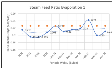
Gambar 3.1 Rasio Steam-to-Feed unit 1
