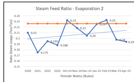
Gambar 3.2 Rasio Steam-to-Feed unit 2
